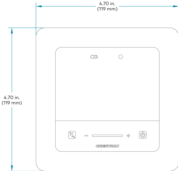
MPC3-101/102/201-RMB with MPC3-201-B installed
