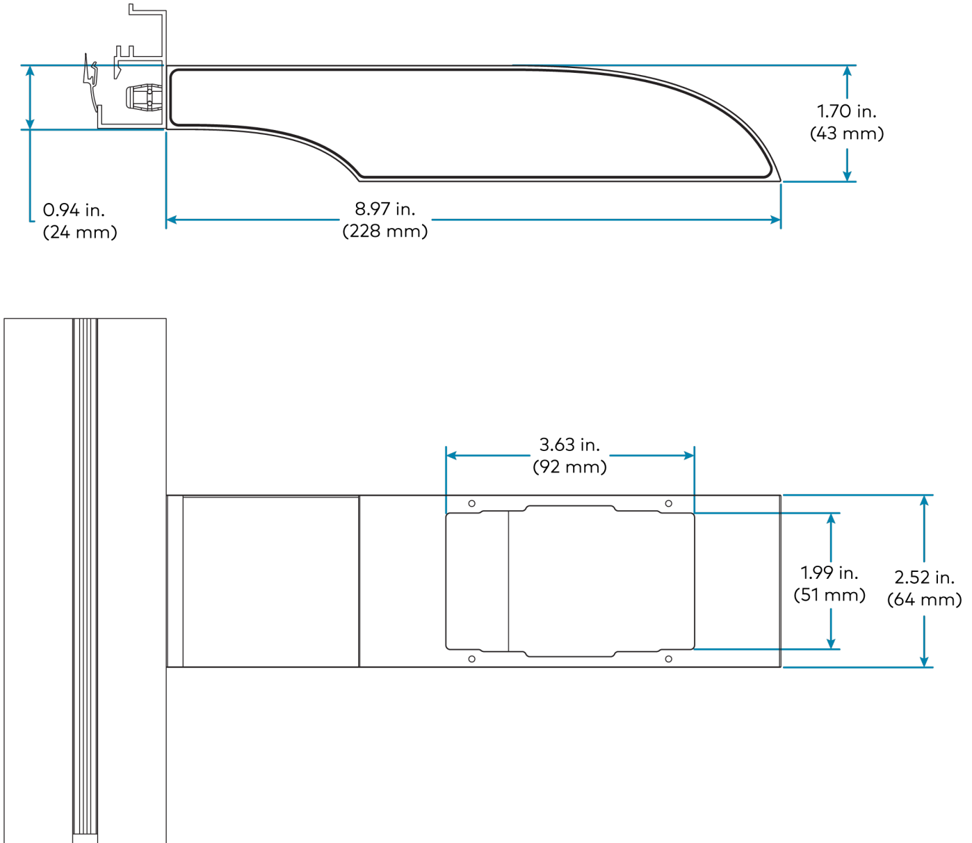
Side Mount Configuration
