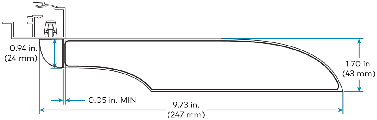
Front Mount Configuration
